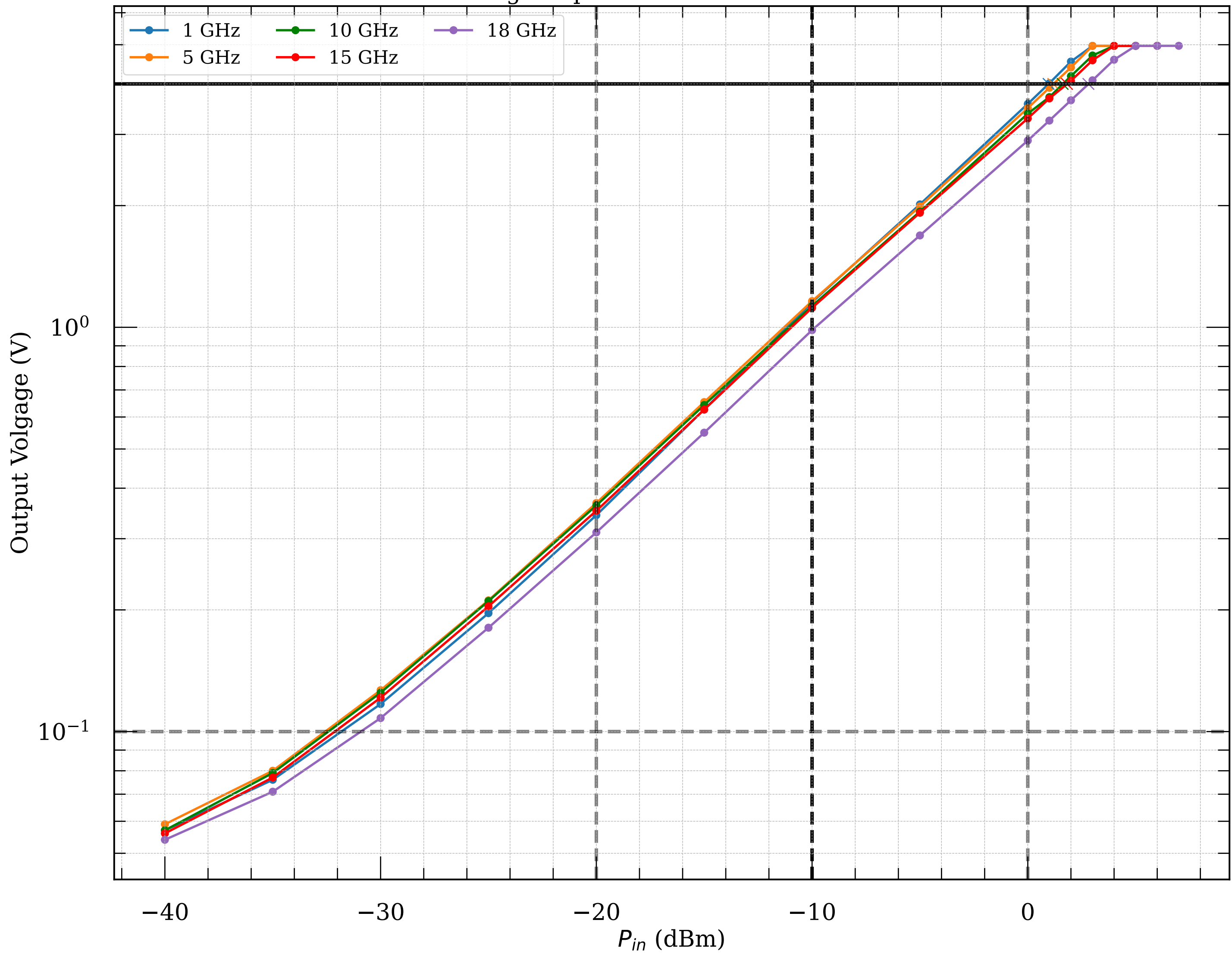
Measured voltage-to-power curve of detector module040v2
